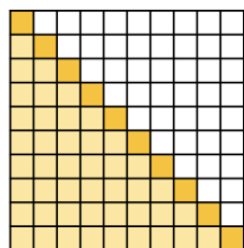
(a) Dense Attention
